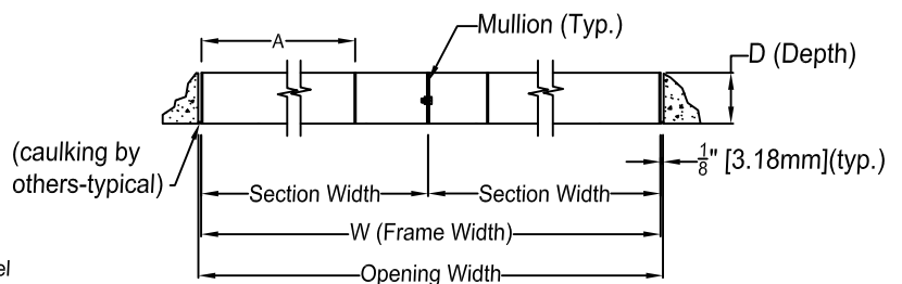
HORIZONTAL SECTION
